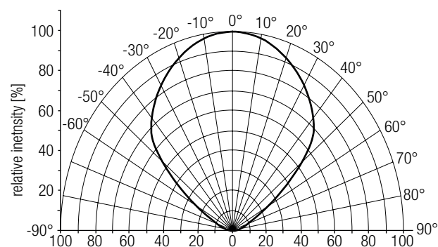
DLA G1 150mm 2000lm 8xx xxx SNC with 90° reflector
