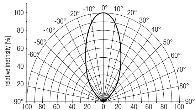
DLA G1 150mm 2000lm 8xx xxx SNC with 60° reflector
